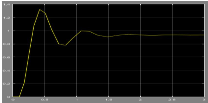
Figure 3: System response at K_u=8.5
