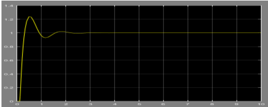
Figure 4: System response with Zeigler-Nichols Tuning
