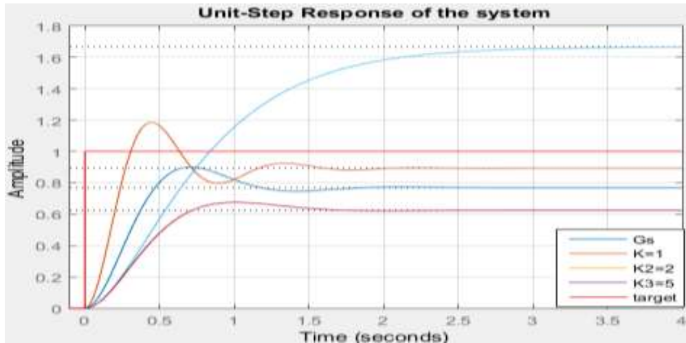
Figure 1: Plot of Transfer Function with Proportional Controller
