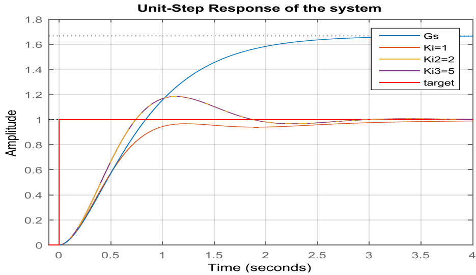
Figure 2: Plot of Transfer Function with Proportional-Integral Controller
