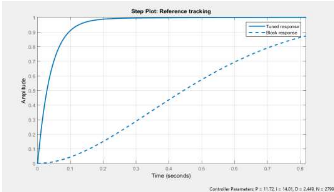
Figure 6: Tuned Response with Auto-tuning
